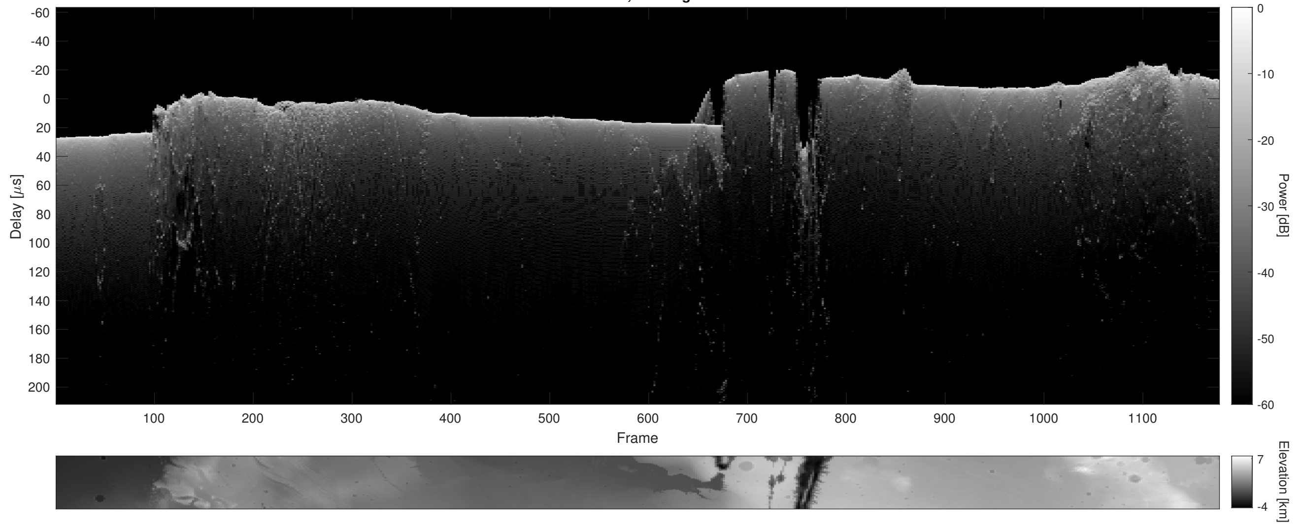
Orbit 9309, Cluttergram
