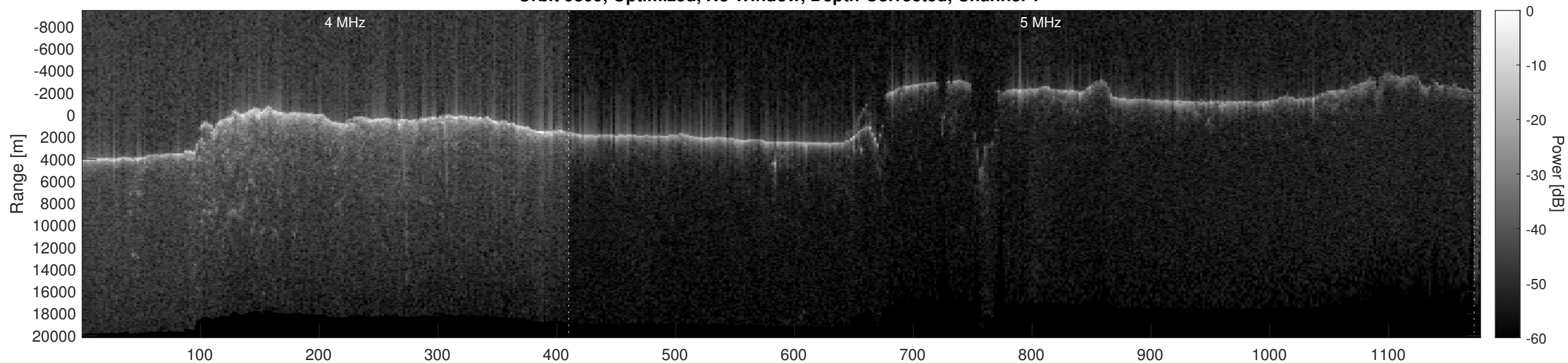
Orbit 9309, Optimized, No Window, Depth-Corrected, Channel 2
