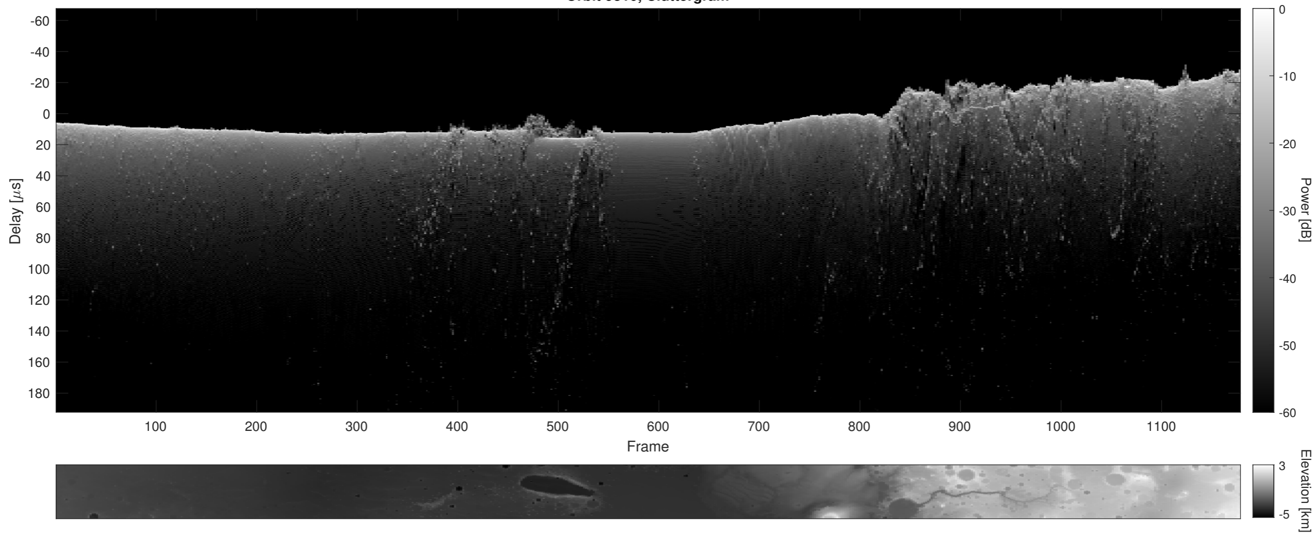
Orbit 9310, Cluttergram
