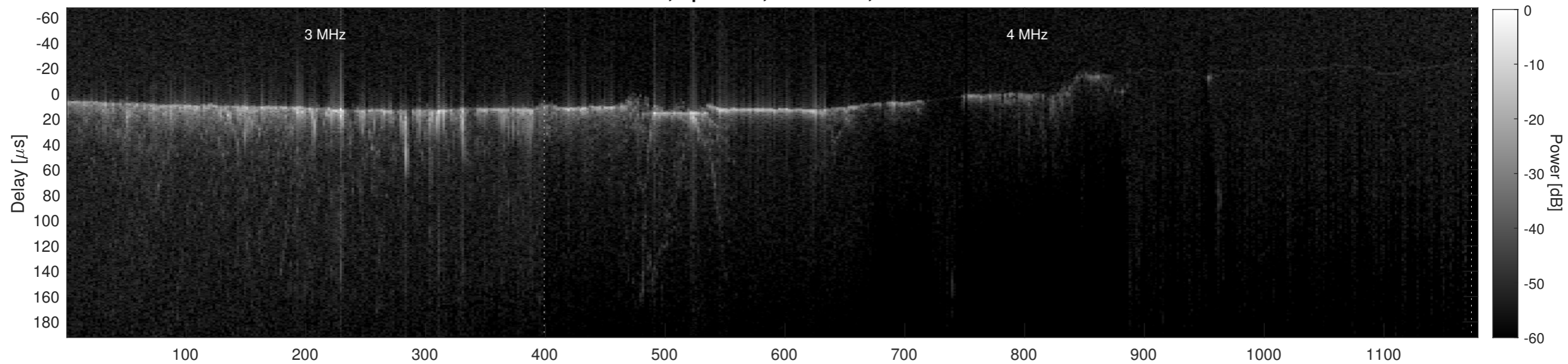
Orbit 9310, Cluttergram
