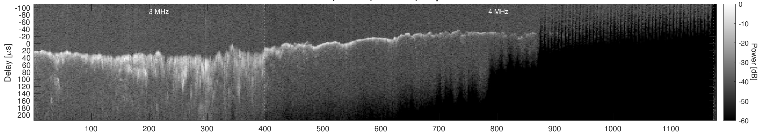
Orbit 9311, Window, Channel 2, Optimized
