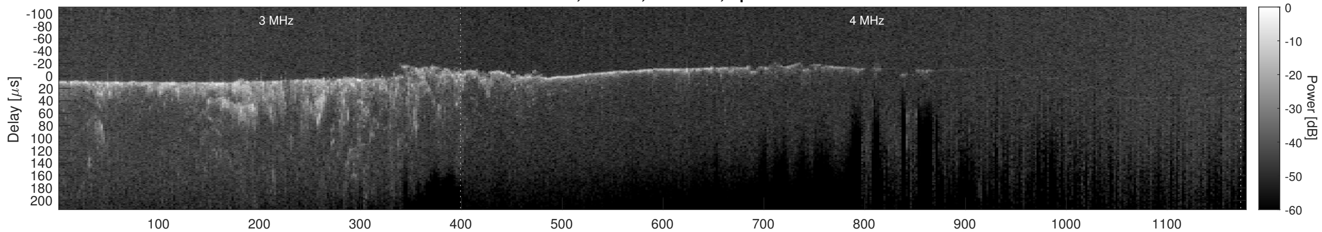
Orbit 9311, Cluttergram
