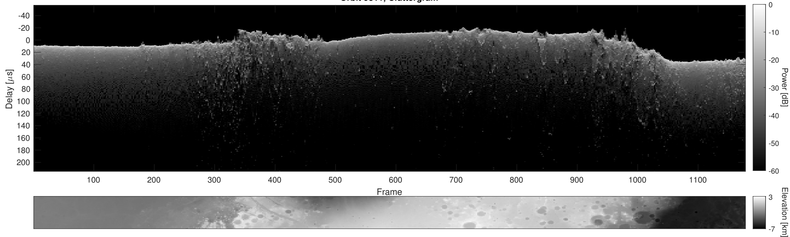
Orbit 9311, Cluttergram
