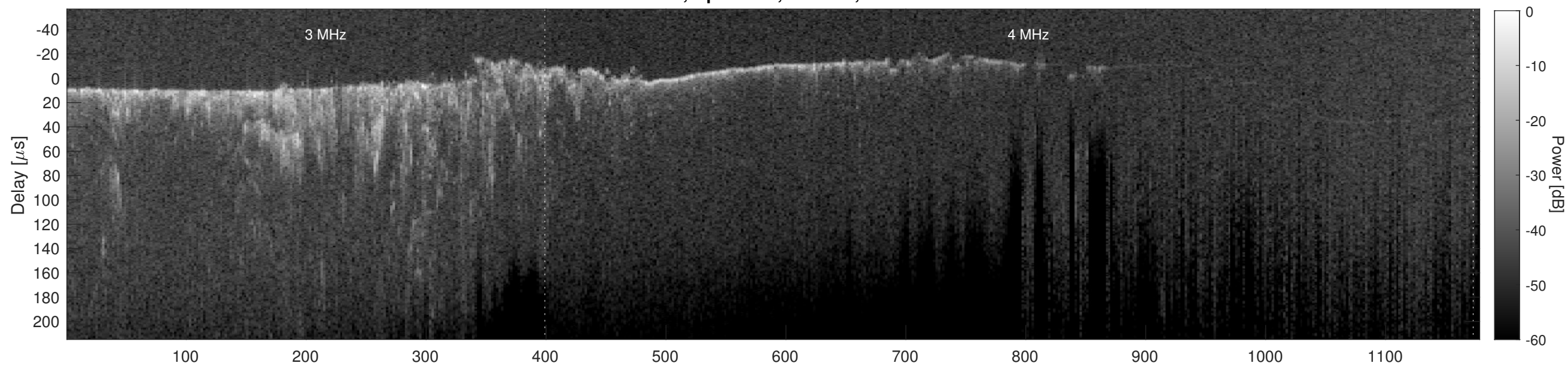
Orbit 9311, Cluttergram
