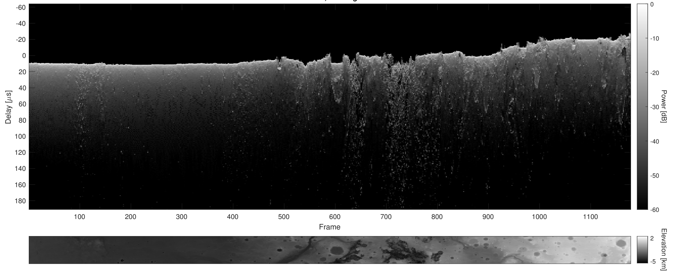
Orbit 9312, Cluttergram
