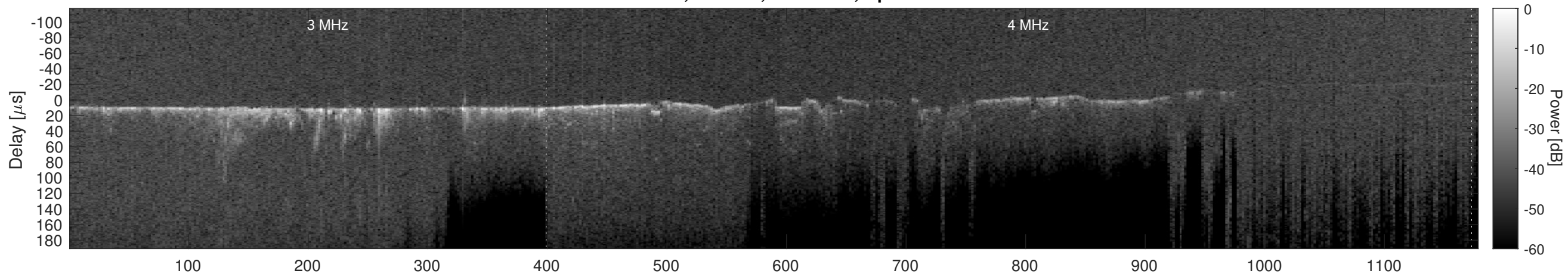
Orbit 9312, Cluttergram
