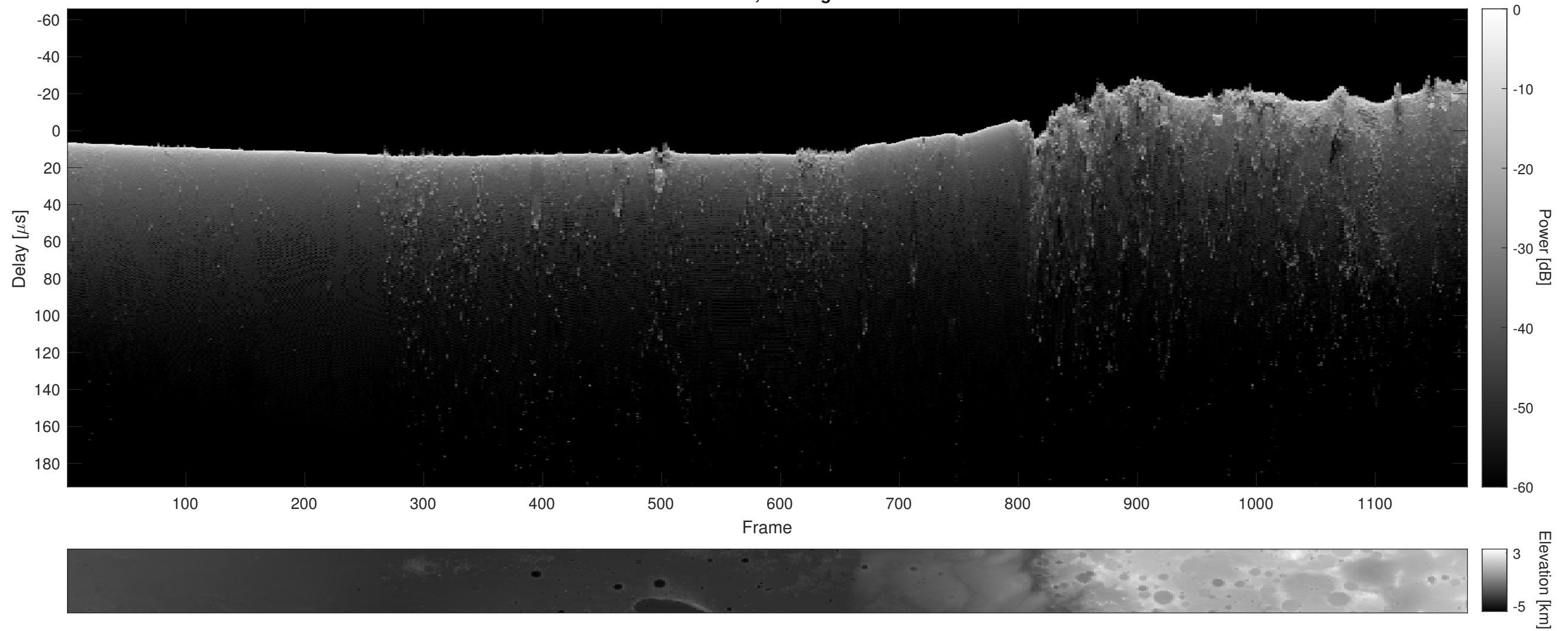
Orbit 9317, Cluttergram
