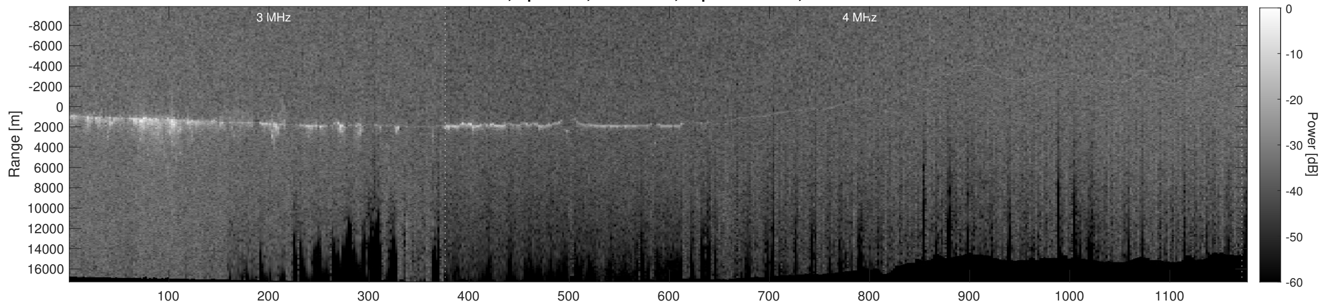
Orbit 9317, Depth-Corrected Cluttergram
