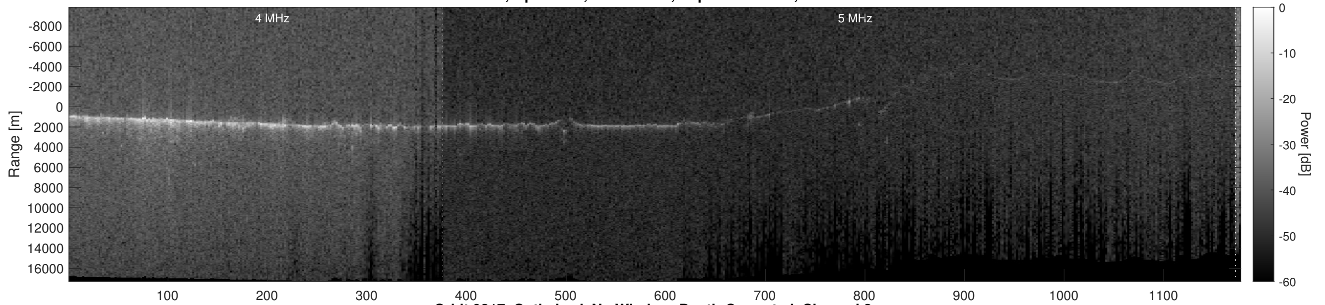
Orbit 9317, Optimized, No Window, Depth-Corrected, Channel 2
