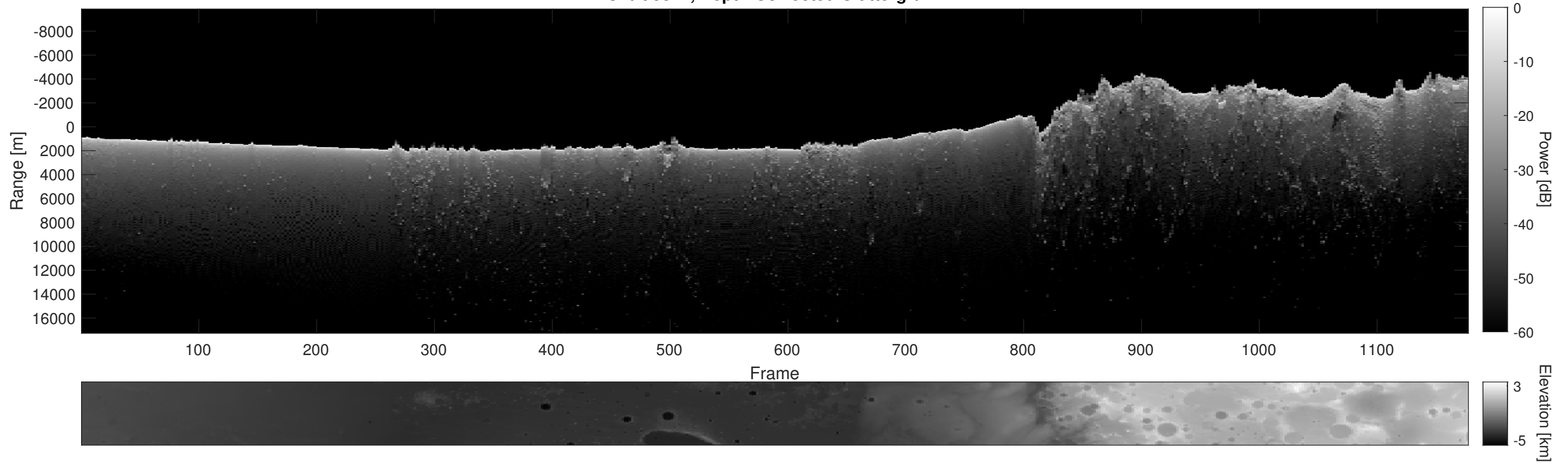
Orbit 9317, Depth-Corrected Cluttergram
