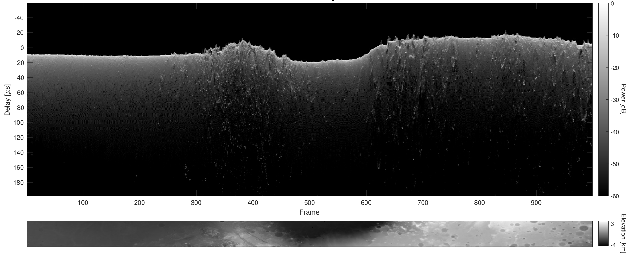
Orbit 9318, Cluttergram
