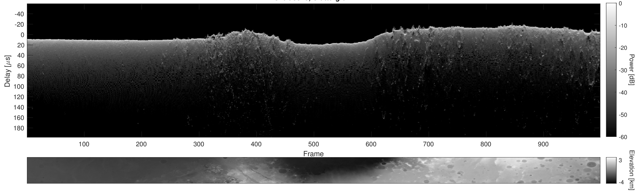
Orbit 9318, Cluttergram
