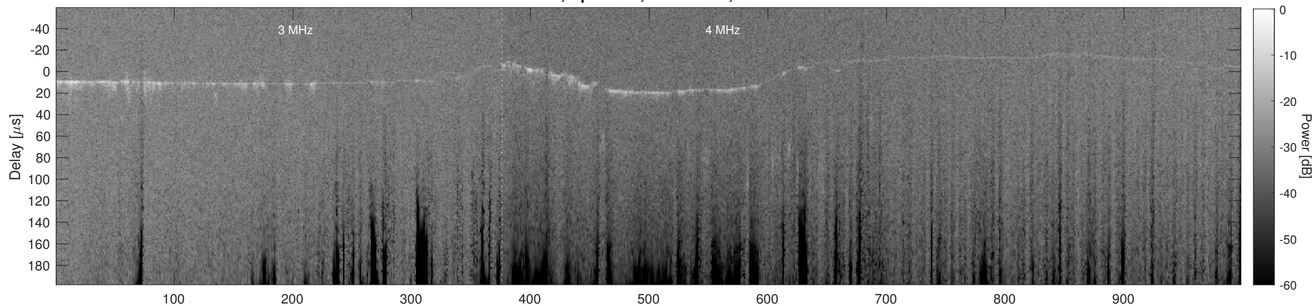
Orbit 9318, Cluttergram
