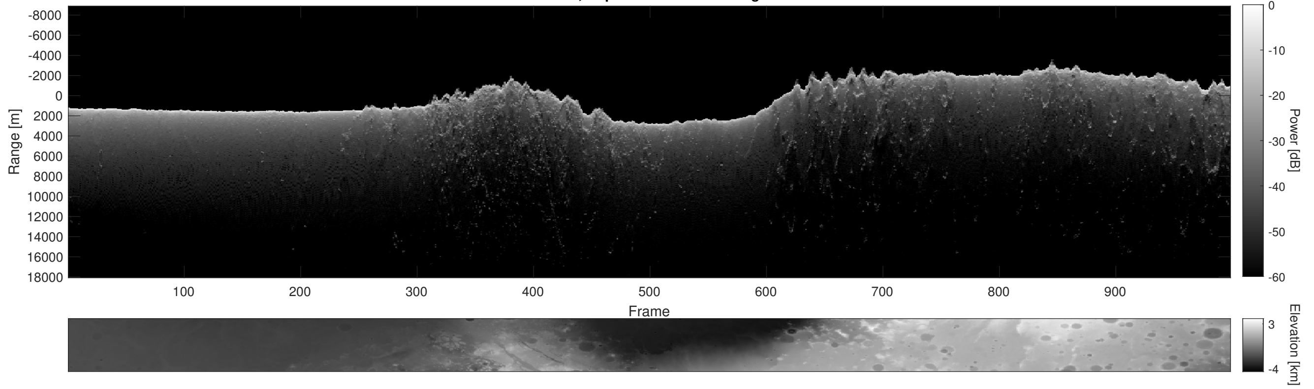
Orbit 9318, Depth-Corrected Cluttergram
