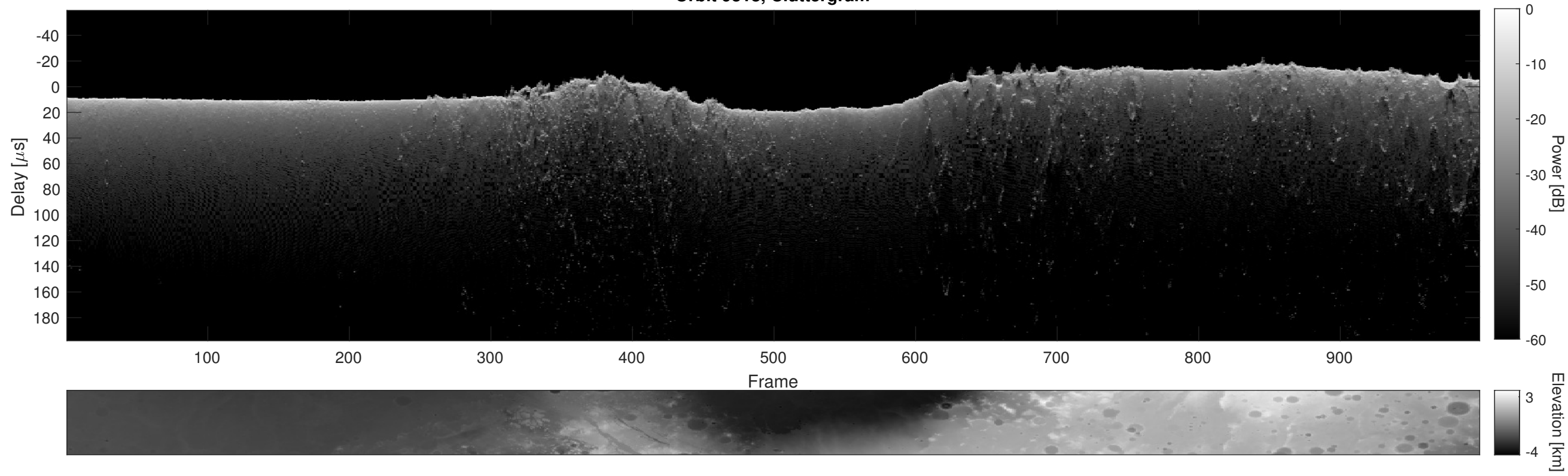
Orbit 9318, Cluttergram
