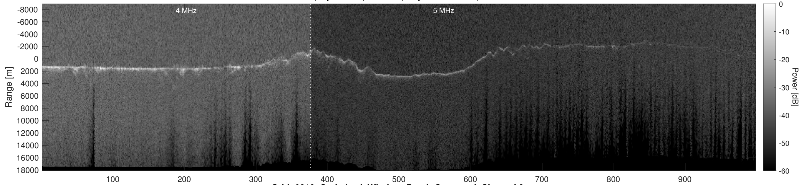
Orbit 9318, Optimized, Window, Depth-Corrected, Channel 2
