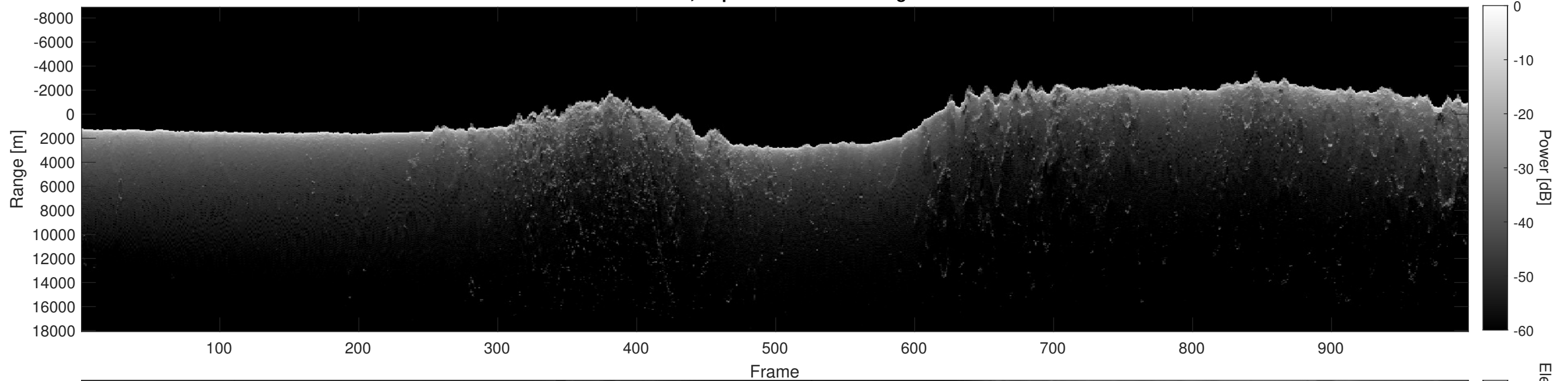
Orbit 9318, Depth-Corrected Cluttergram
