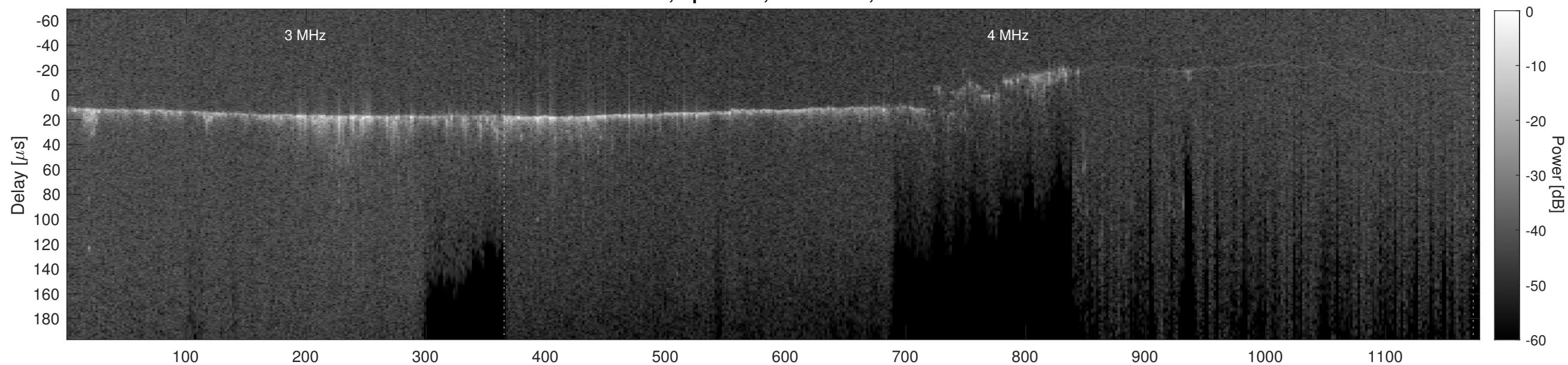
Orbit 9321, Cluttergram
