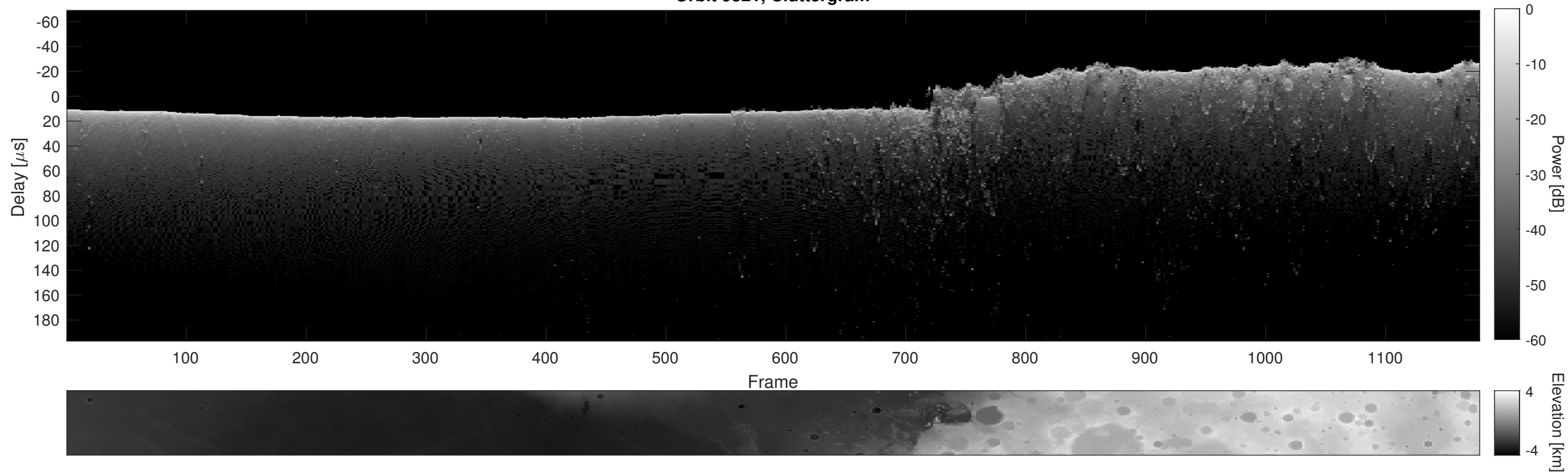
Orbit 9321, Cluttergram
