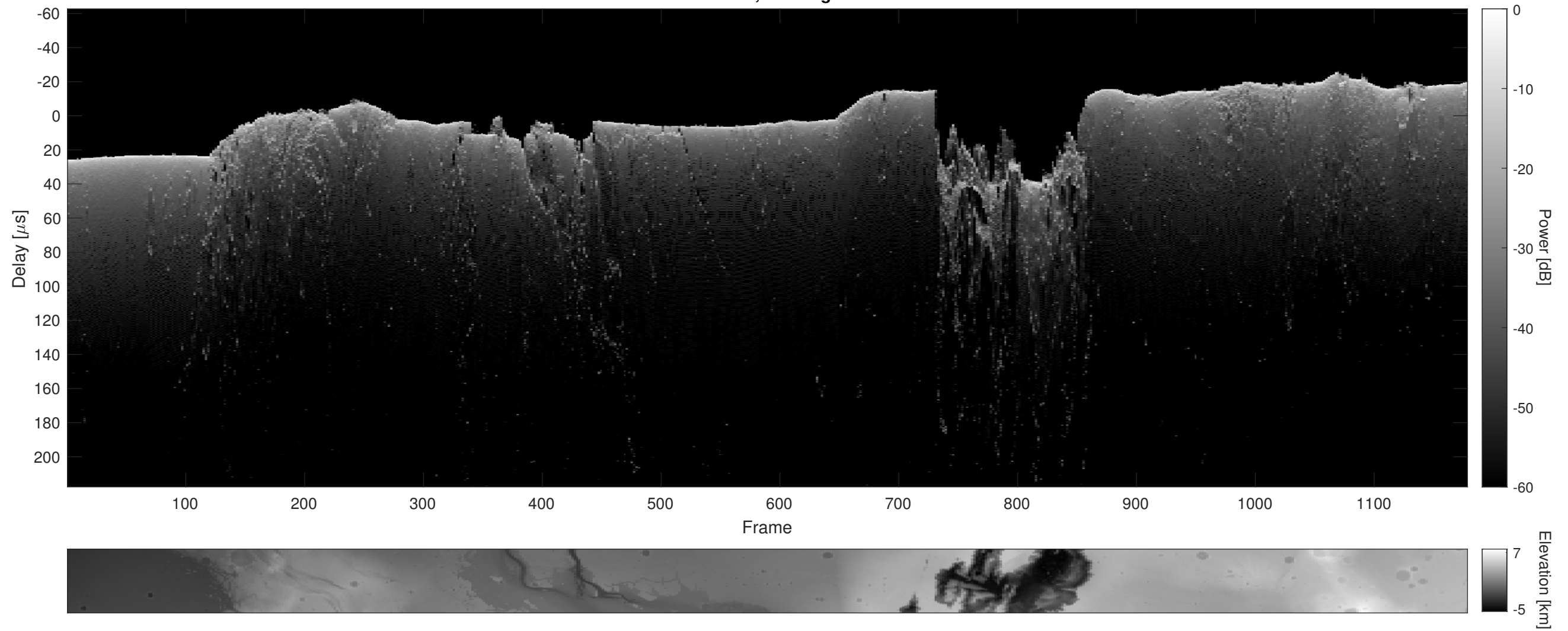
Orbit 9323, Cluttergram
