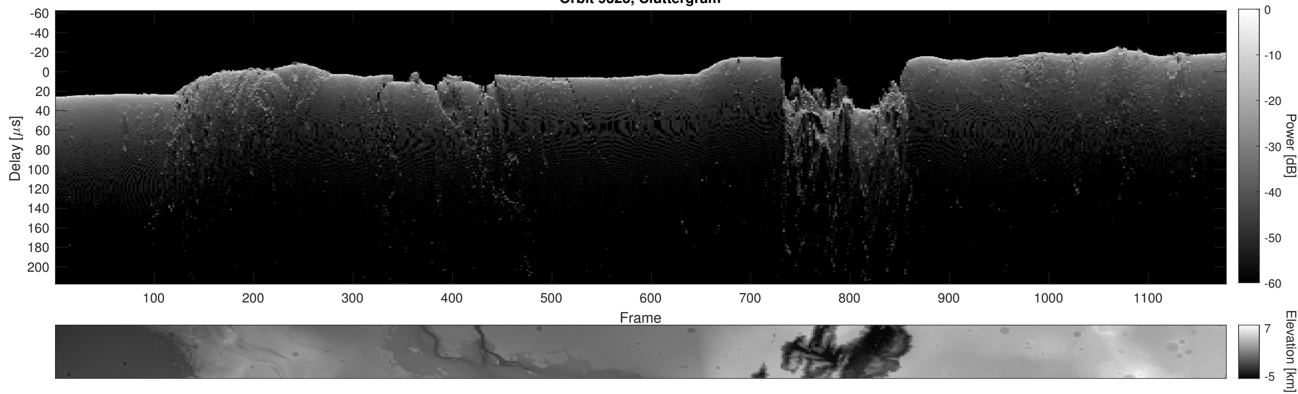
Orbit 9323, Cluttergram
