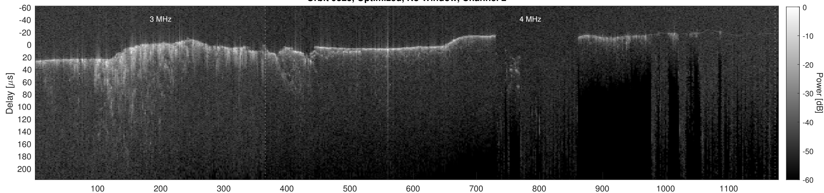
Orbit 9323, Cluttergram
