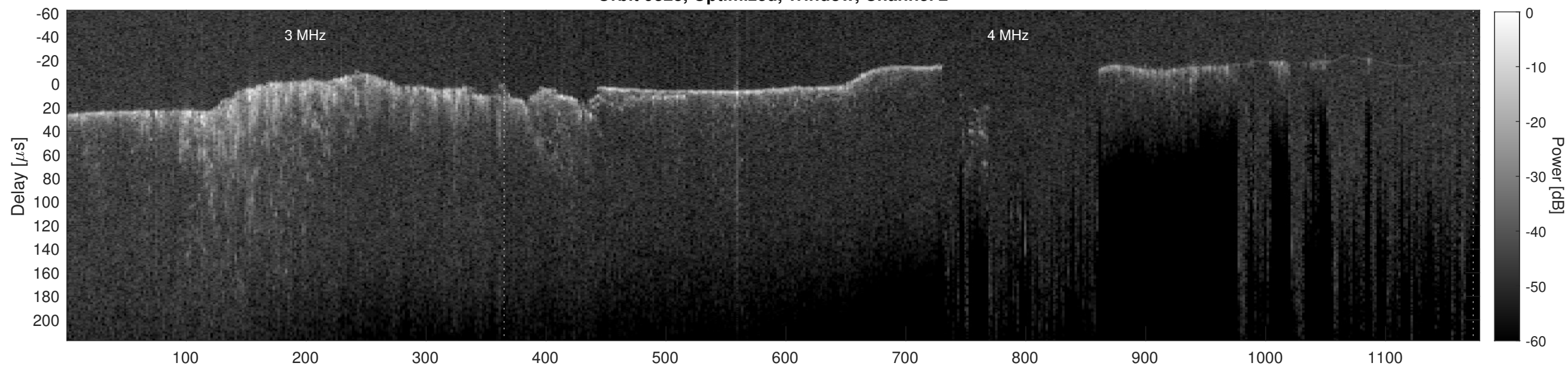
Orbit 9323, Cluttergram
