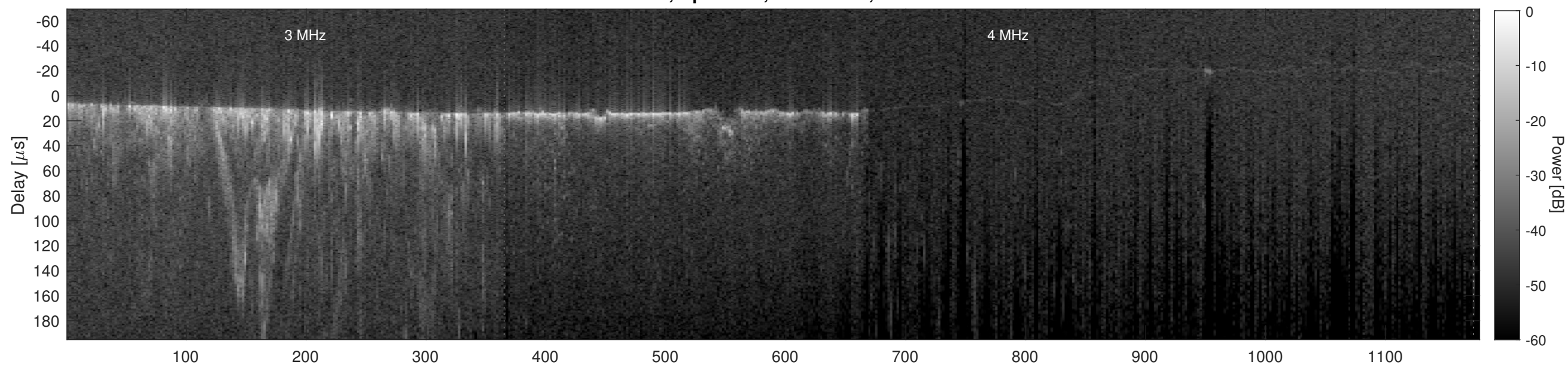
Orbit 9324, Cluttergram
