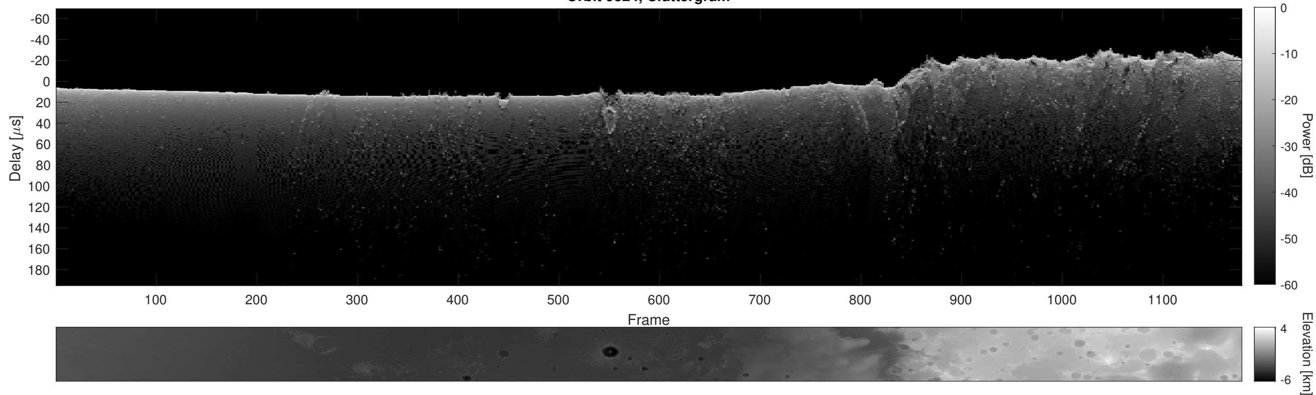
Orbit 9324, Cluttergram
