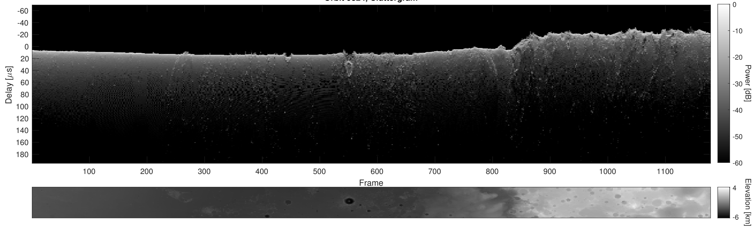
Orbit 9324, Cluttergram
