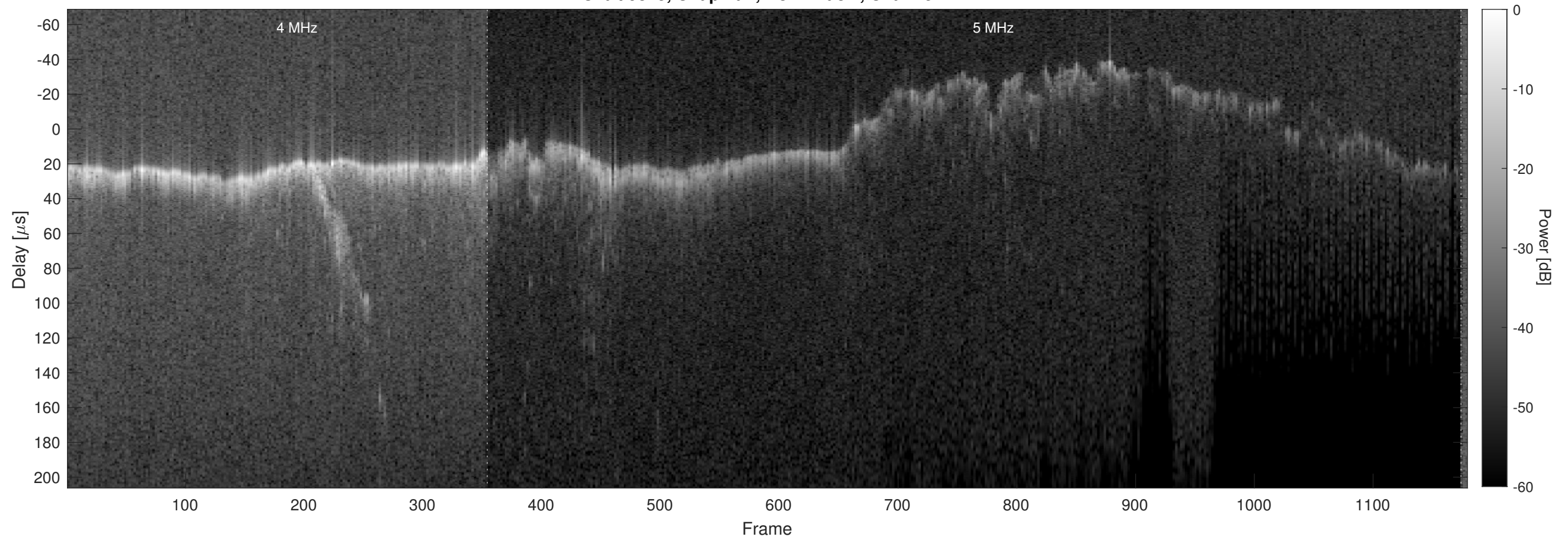
Orbit 9325, Chapman, No Window, Channel 2
