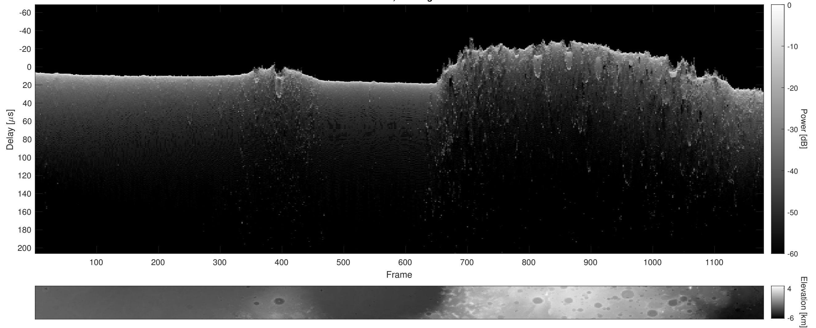
Orbit 9325, Cluttergram
