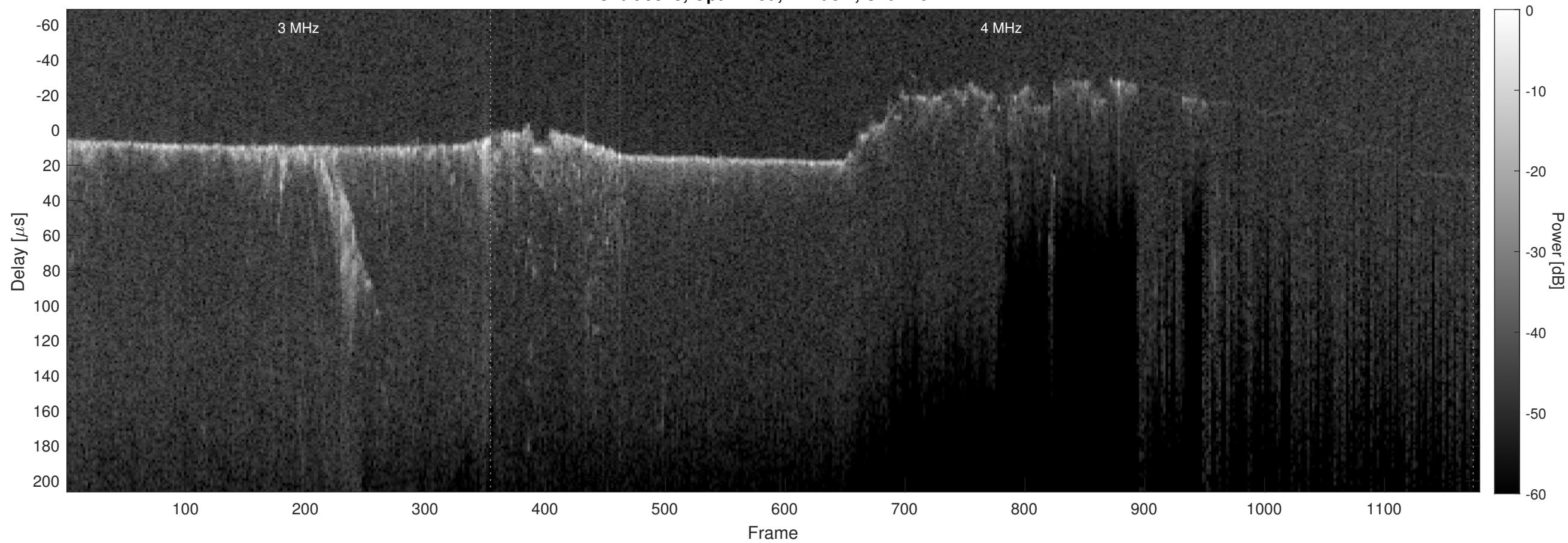
Orbit 9325, Optimized, Window, Channel 2
