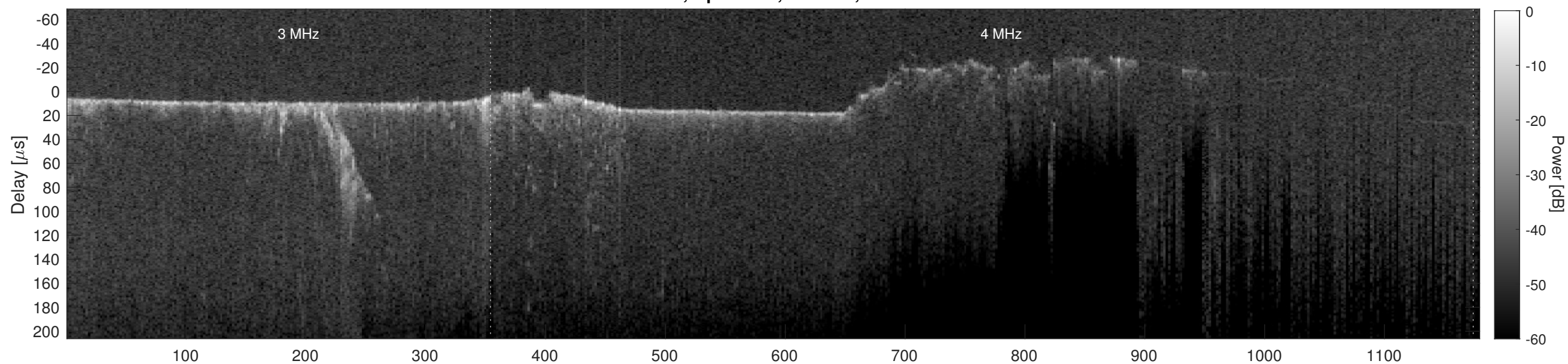
Orbit 9325, Cluttergram
