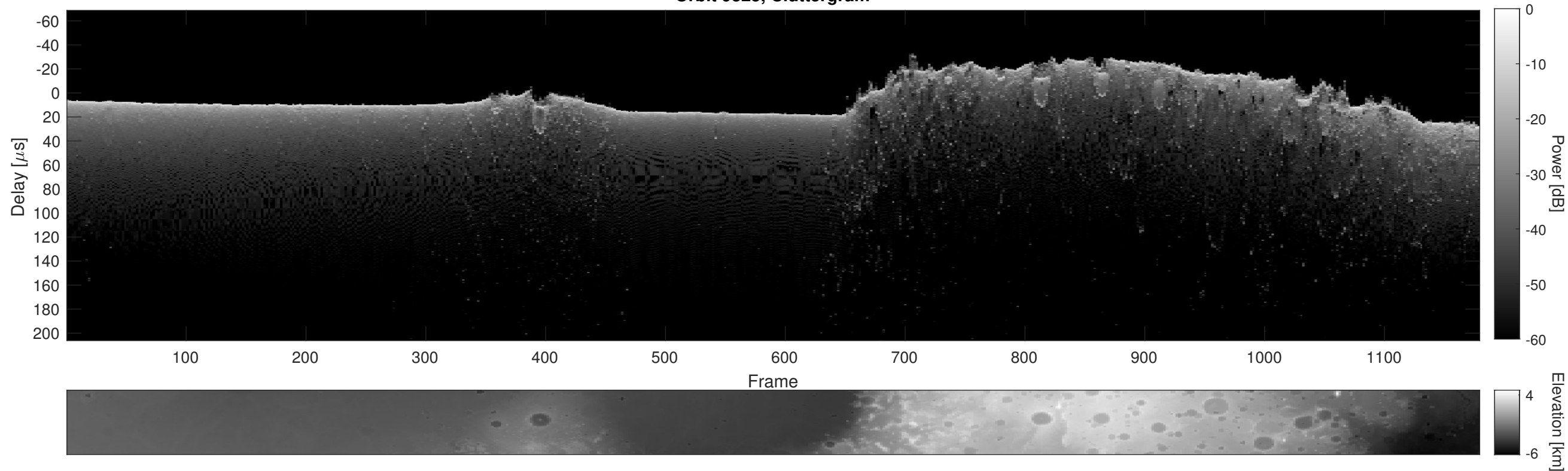
Orbit 9325, Cluttergram
