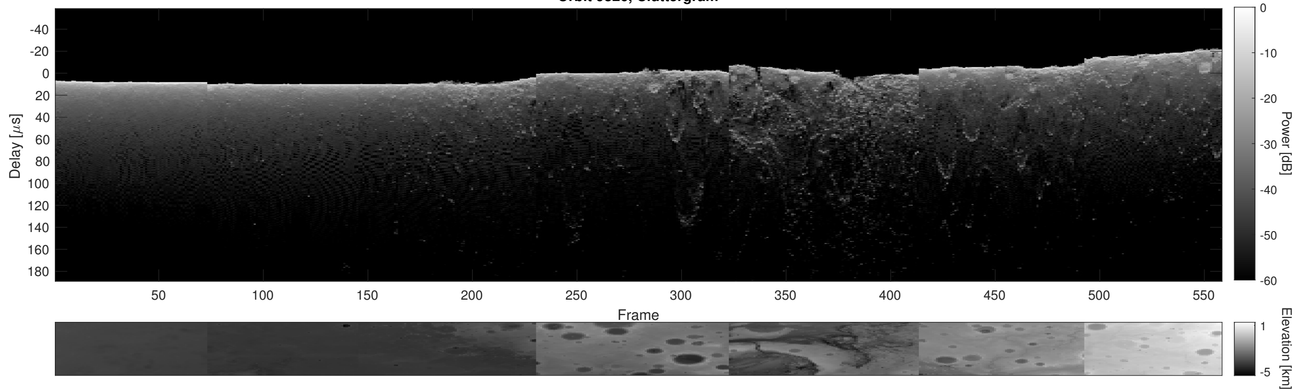
Orbit 9326, Cluttergram
