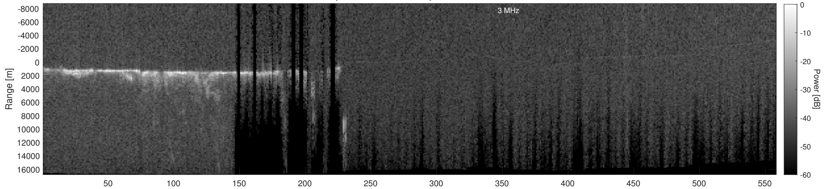
Orbit 9326, Depth-Corrected Cluttergram
