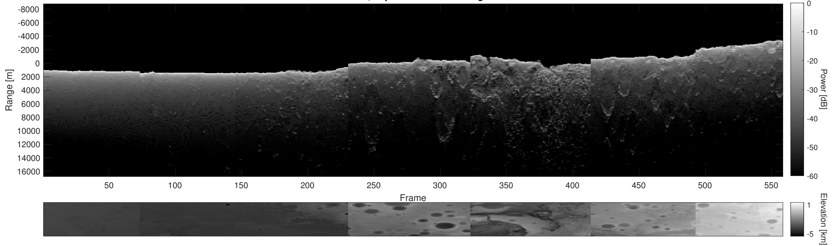
Orbit 9326, Depth-Corrected Cluttergram
