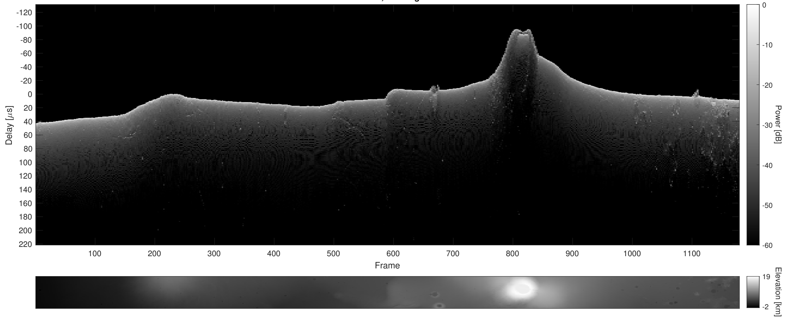
Orbit 9327, Cluttergram
