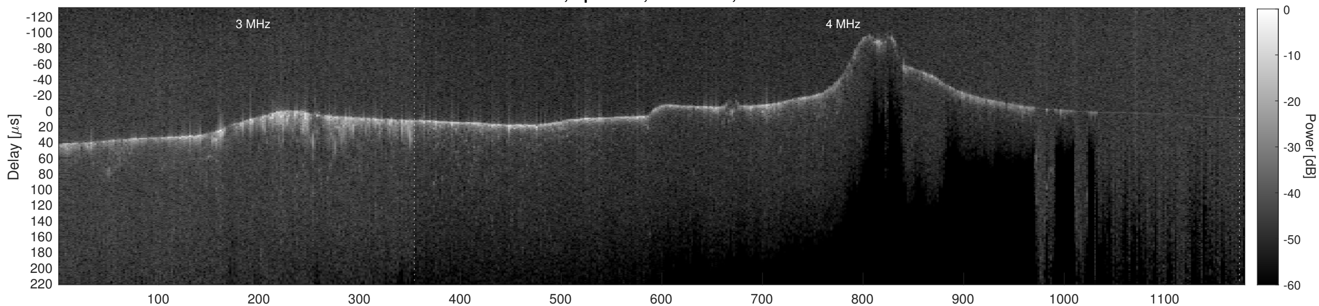
Orbit 9327, Cluttergram
