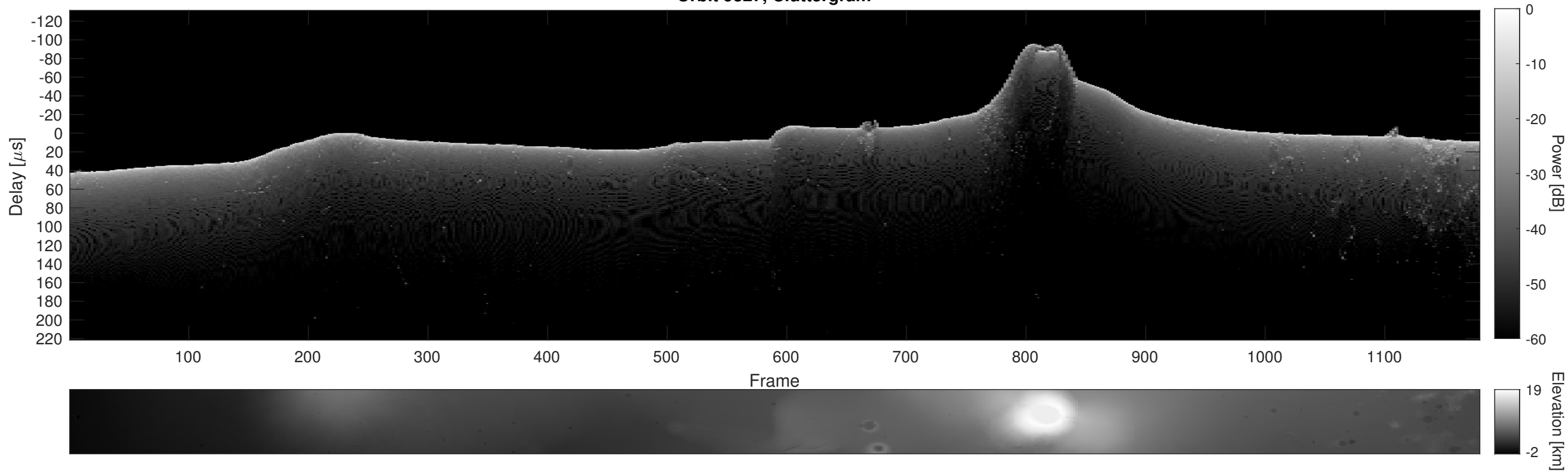
Orbit 9327, Cluttergram
