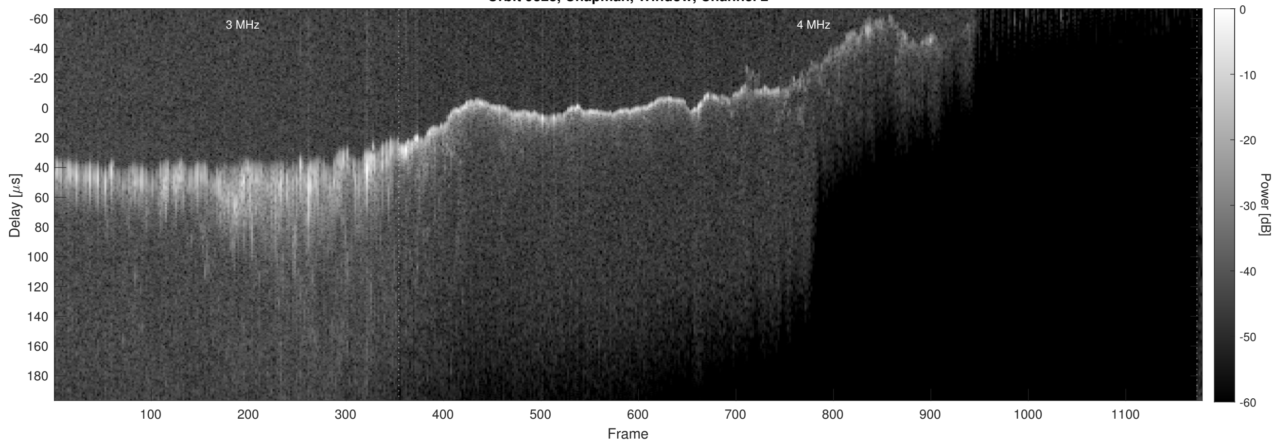
Orbit 9328, Chapman, Window, Channel 2
