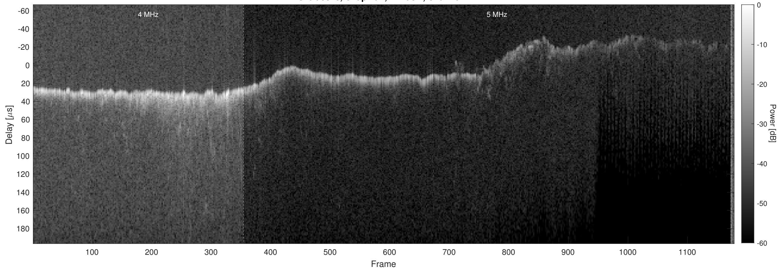
Orbit 9328, Chapman, Window, Channel 2
