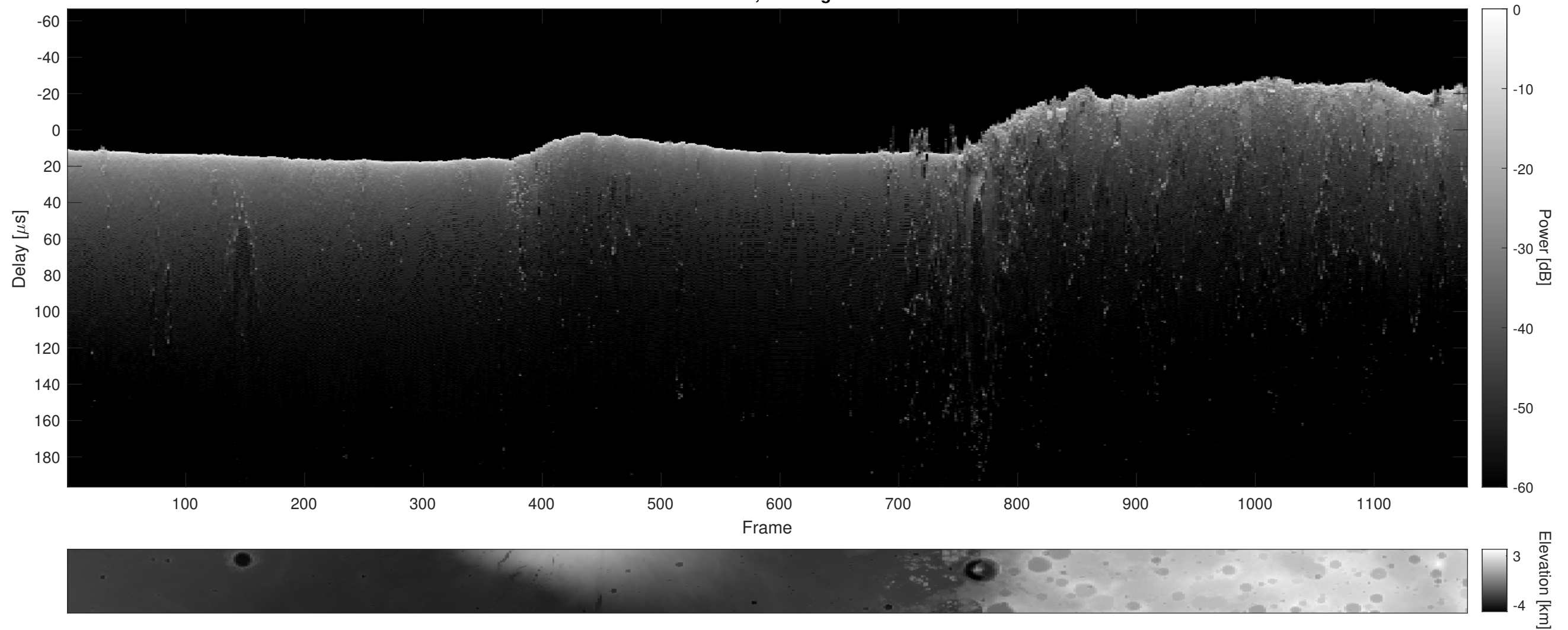
Orbit 9328, Cluttergram
