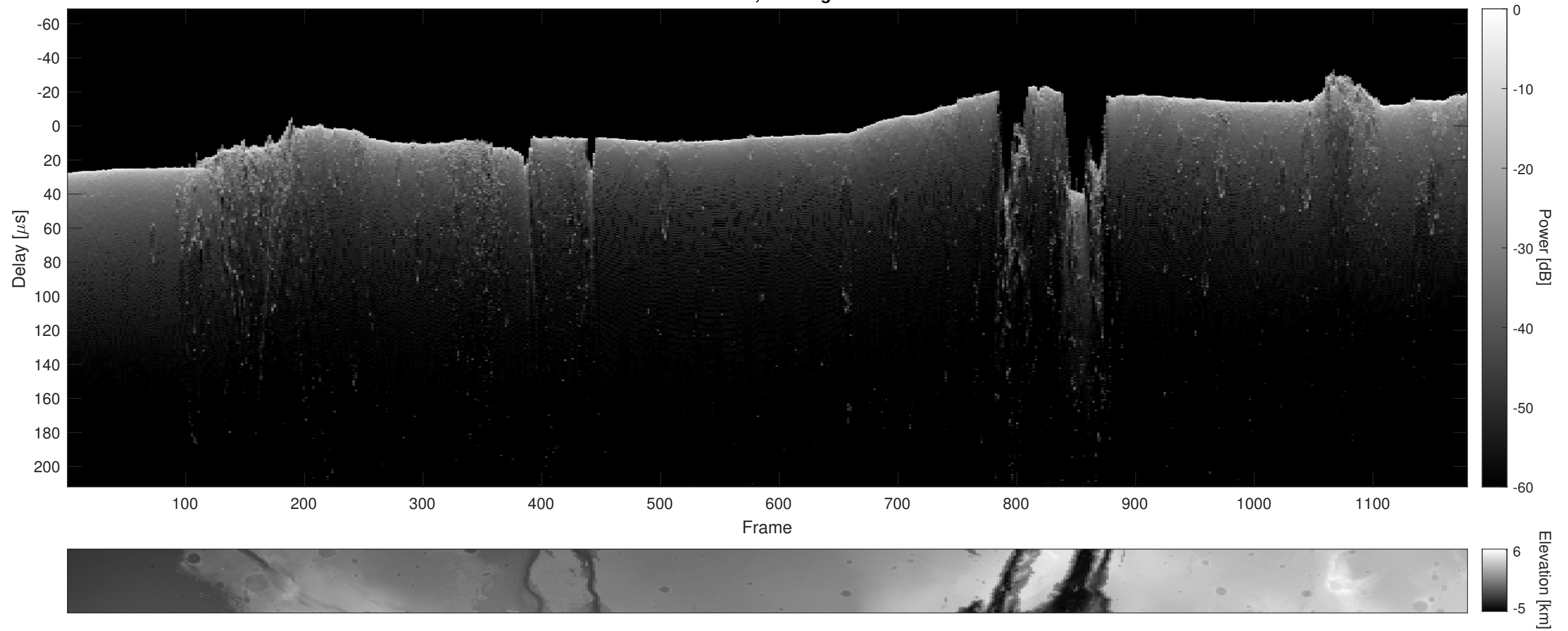
Orbit 9330, Cluttergram
