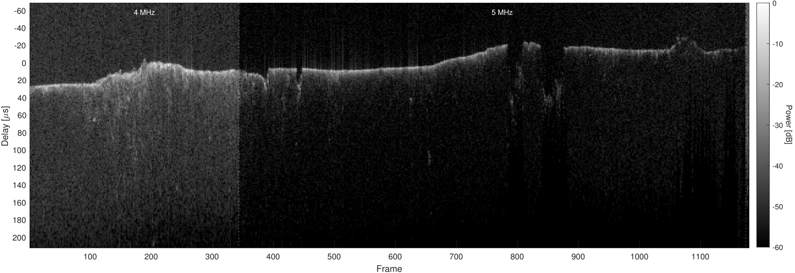
Orbit 9330, Optimized, Window, Channel 2
