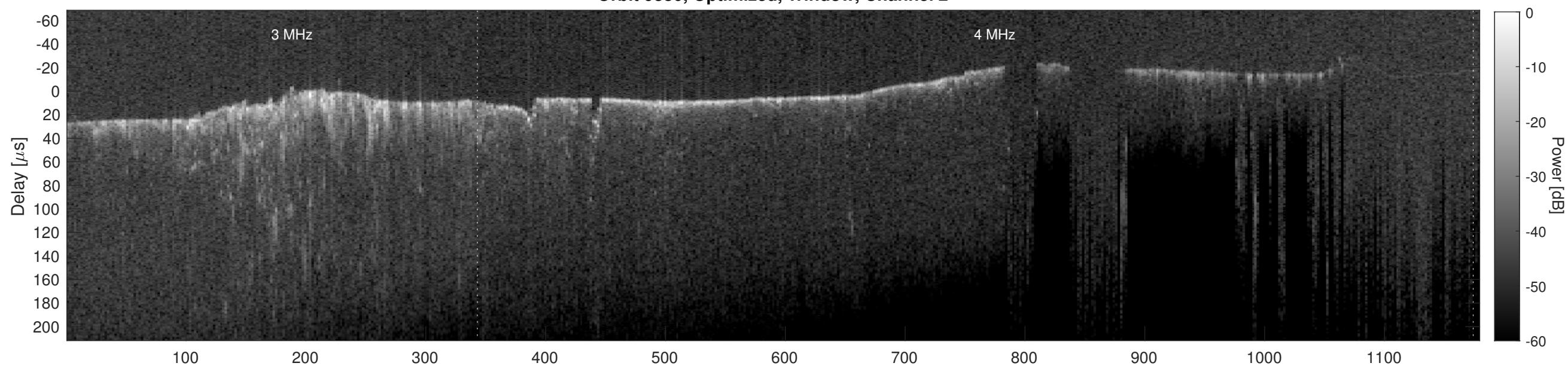
Orbit 9330, Cluttergram
