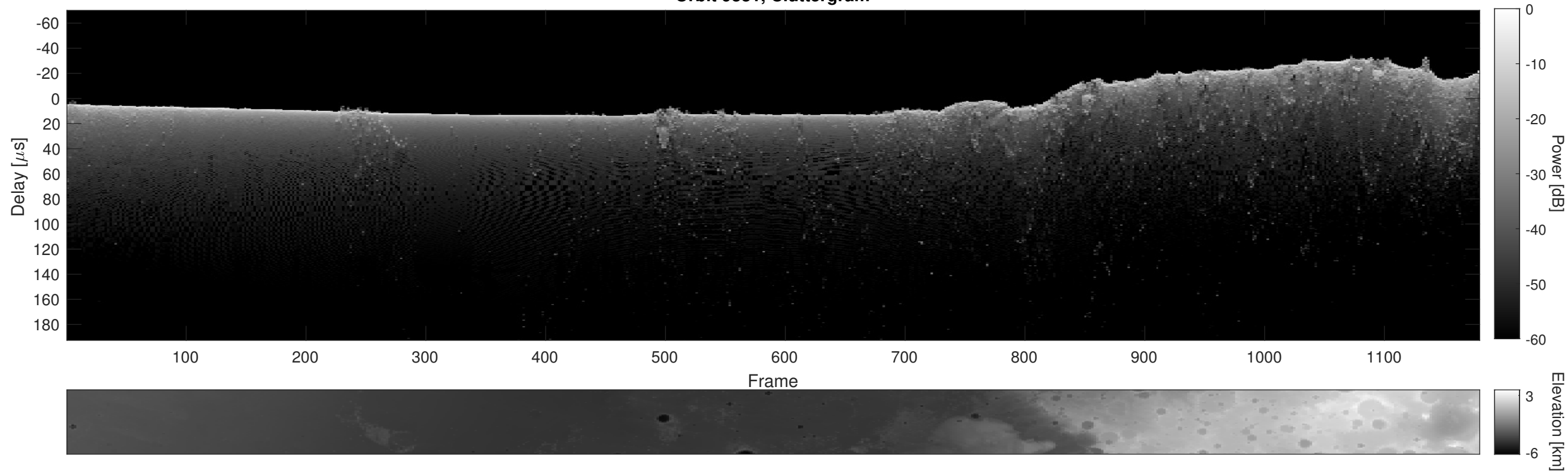
Orbit 9331, Cluttergram
