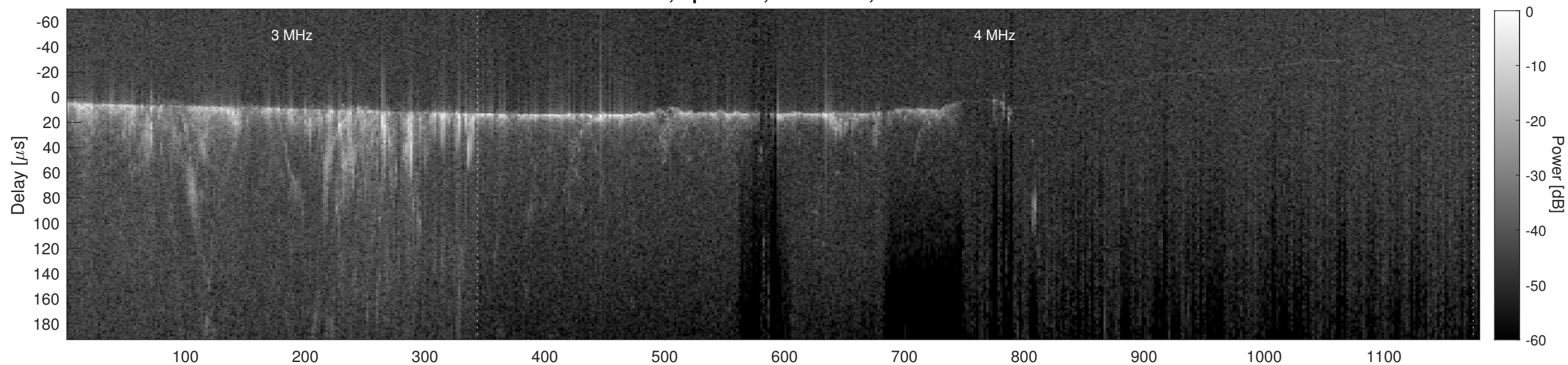
Orbit 9331, Cluttergram
