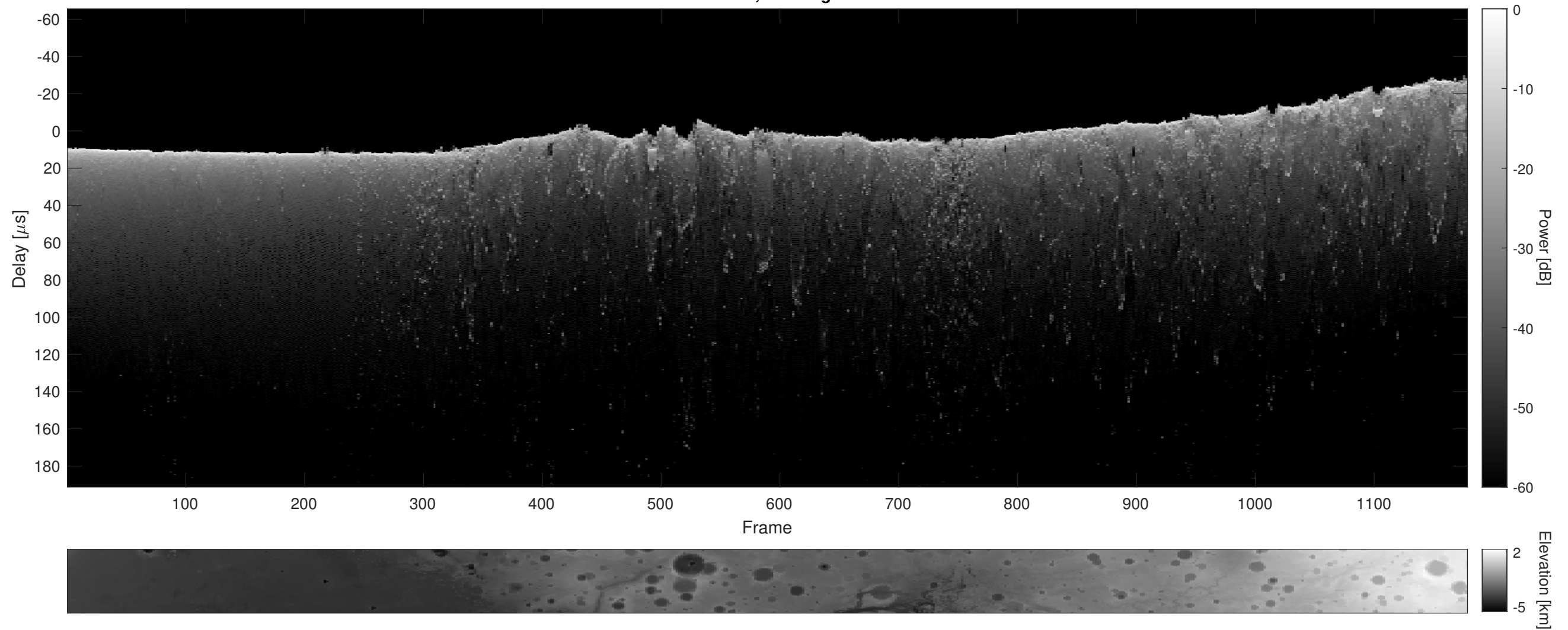
Orbit 9333, Cluttergram
