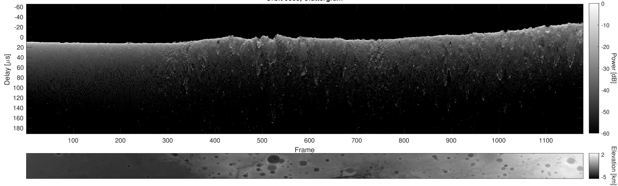
Orbit 9333, Cluttergram
