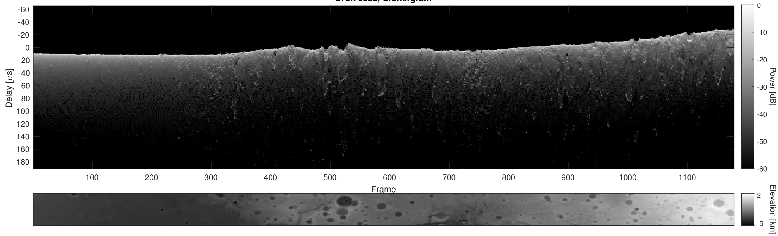
Orbit 9333, Cluttergram
