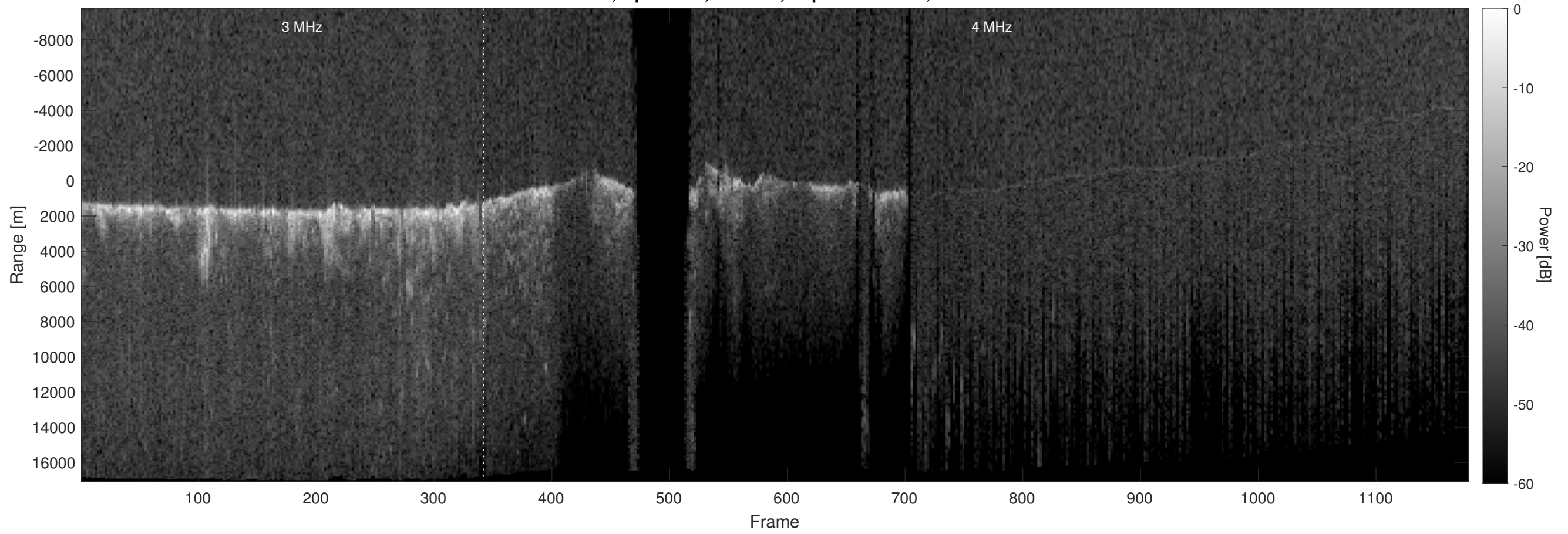
Orbit 9333, Optimized, Window, Depth-Corrected, Channel 2
