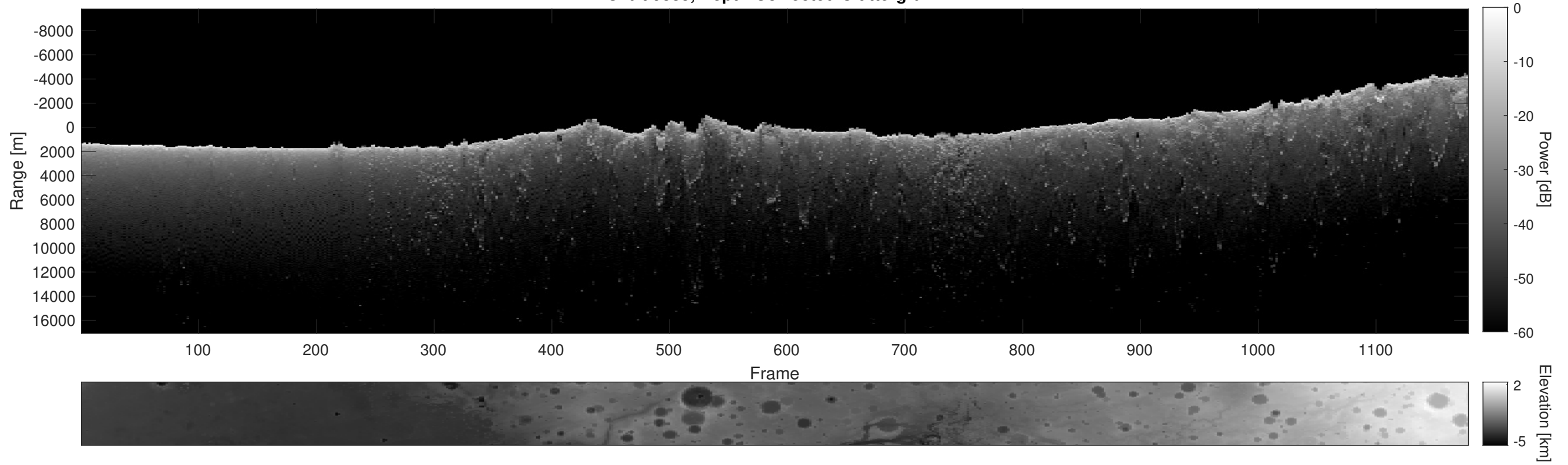
Orbit 9333, Depth-Corrected Cluttergram
