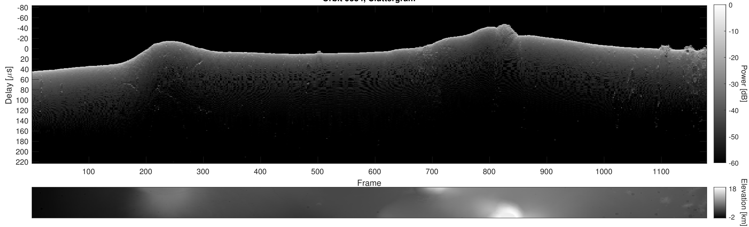
Orbit 9334, Cluttergram
