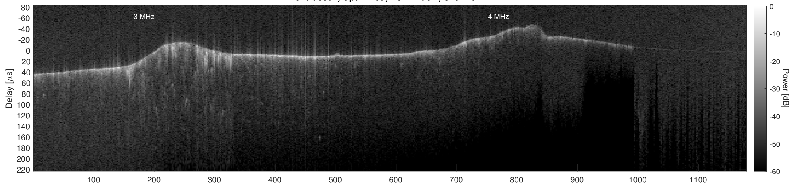
Orbit 9334, Cluttergram
