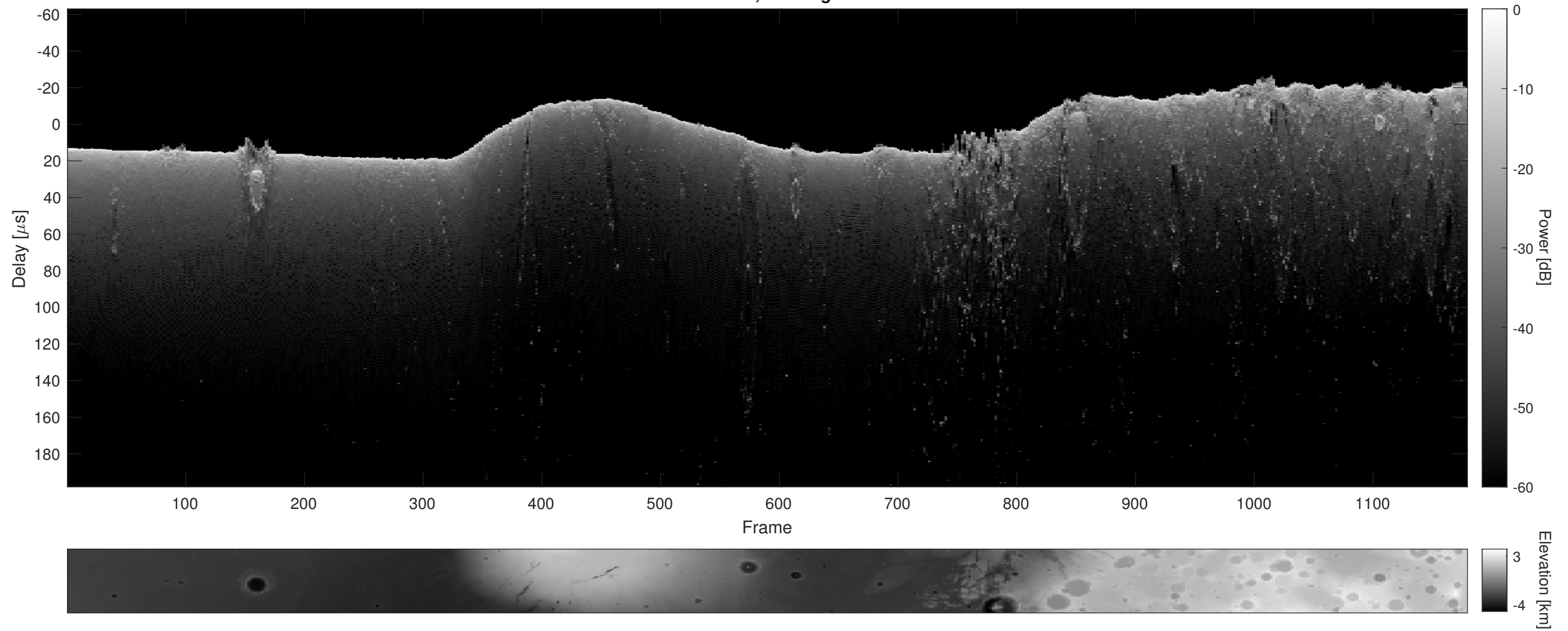
Orbit 9335, Cluttergram
