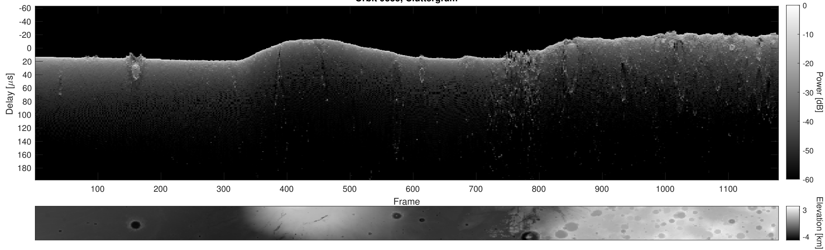
Orbit 9335, Cluttergram
