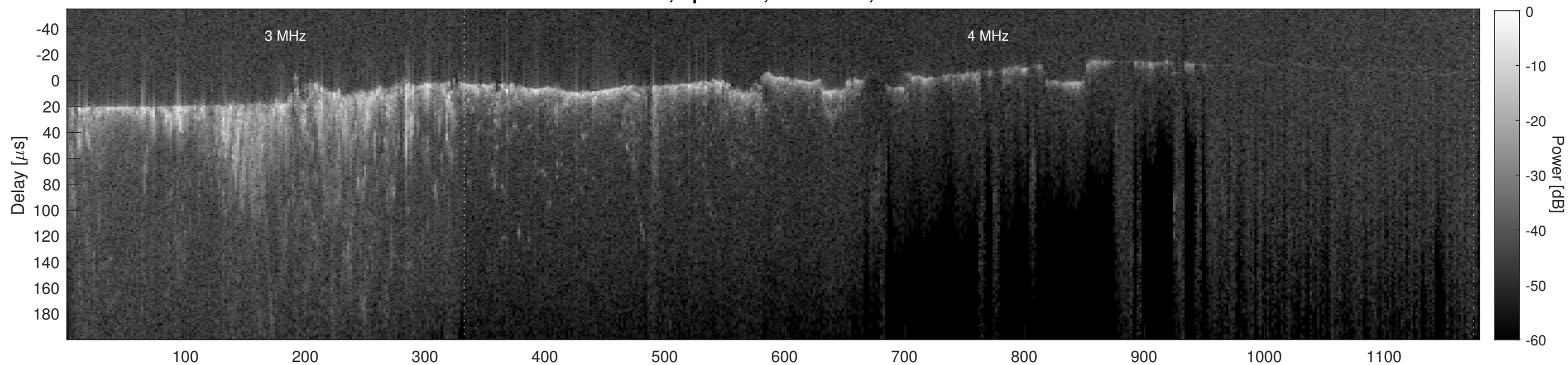
Orbit 9336, Cluttergram
