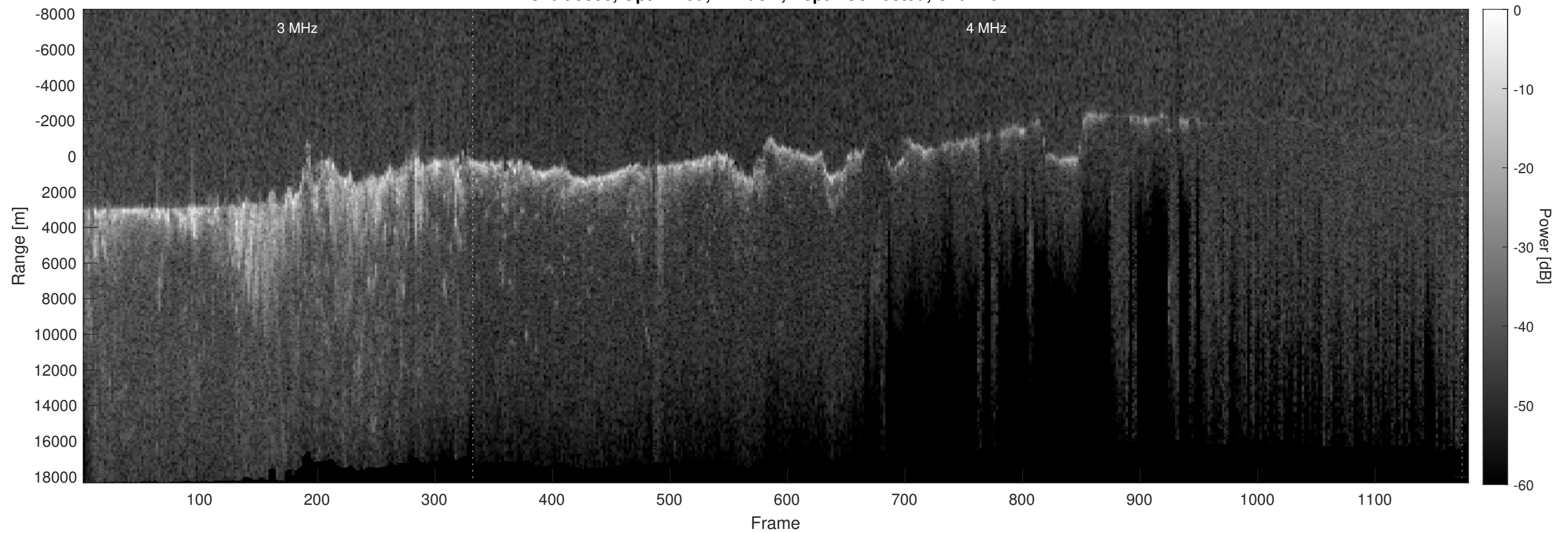
Orbit 9336, Optimized, Window, Depth-Corrected, Channel 2
