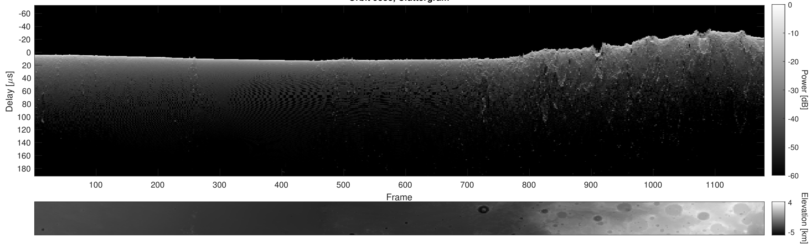
Orbit 9338, Cluttergram
