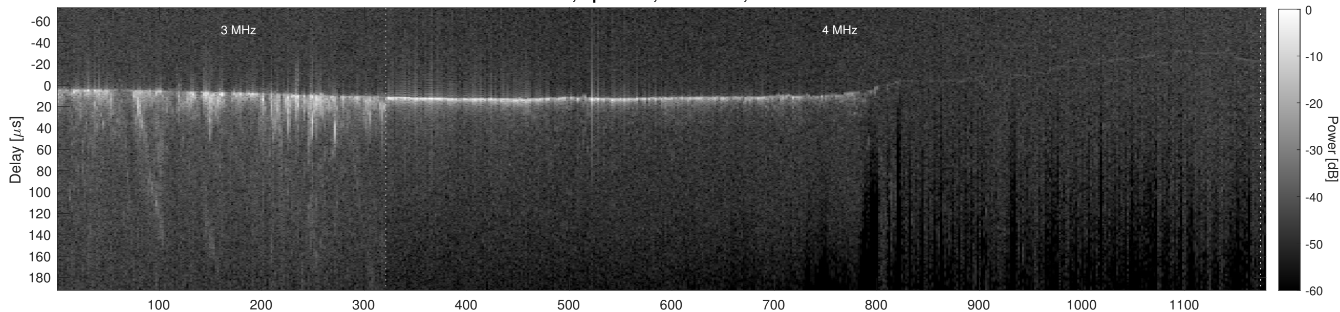
Orbit 9338, Cluttergram
