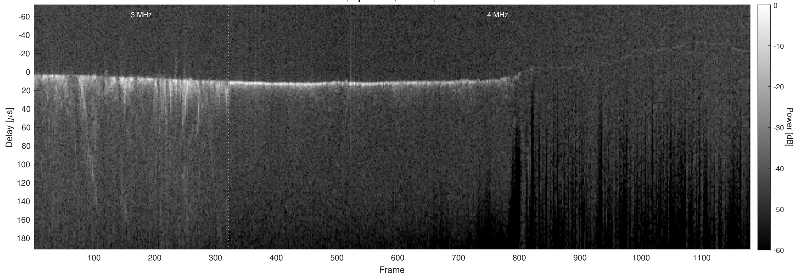
Orbit 9338, Optimized, Window, Channel 2
