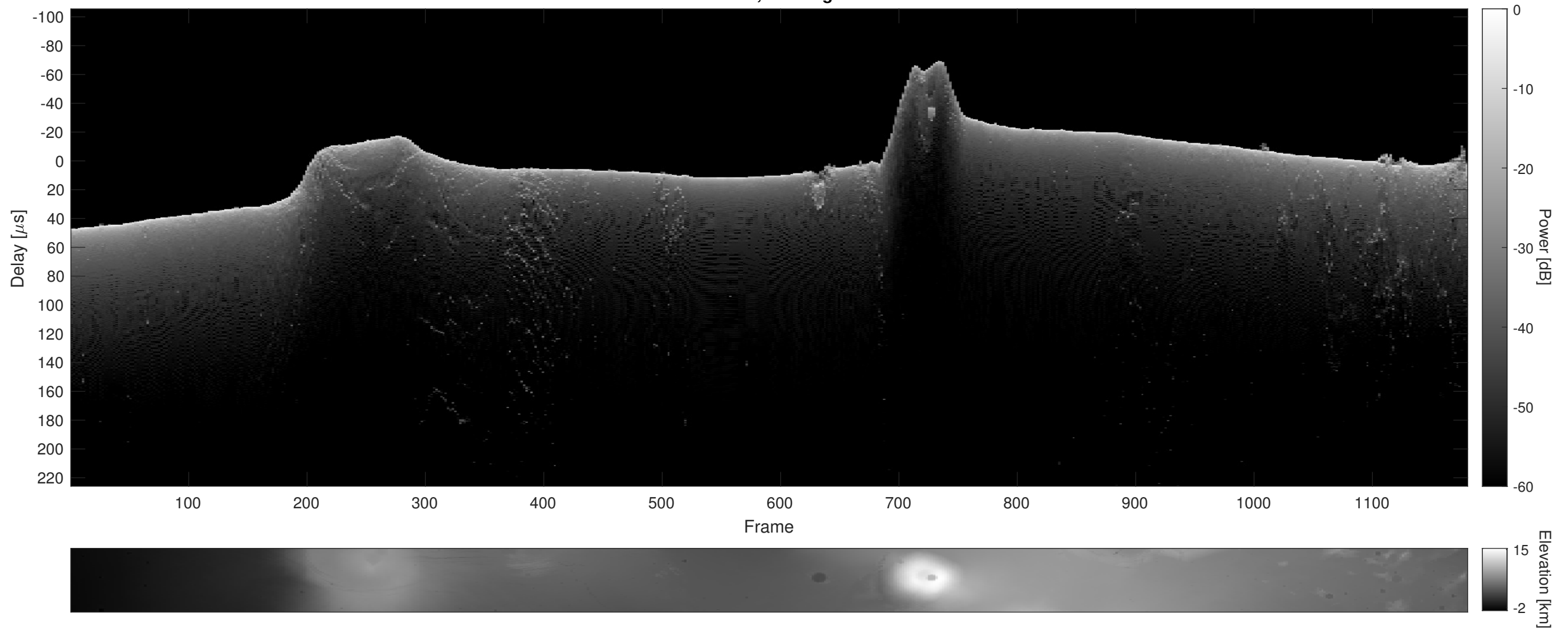
Orbit 9341, Cluttergram
