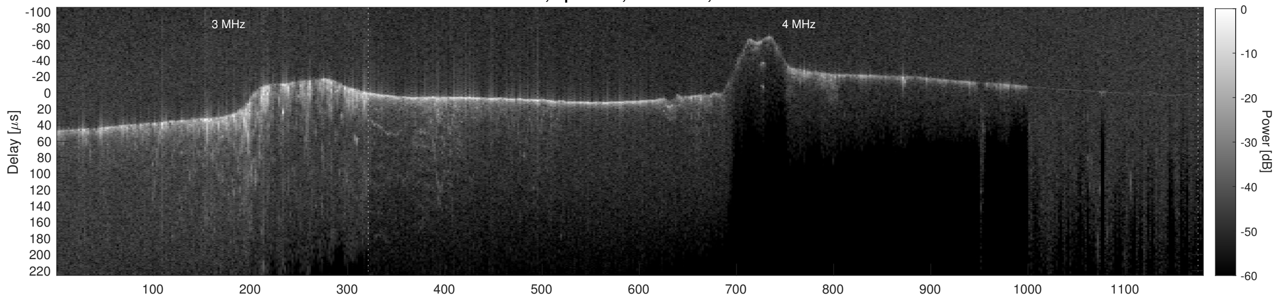
Orbit 9341, Cluttergram
