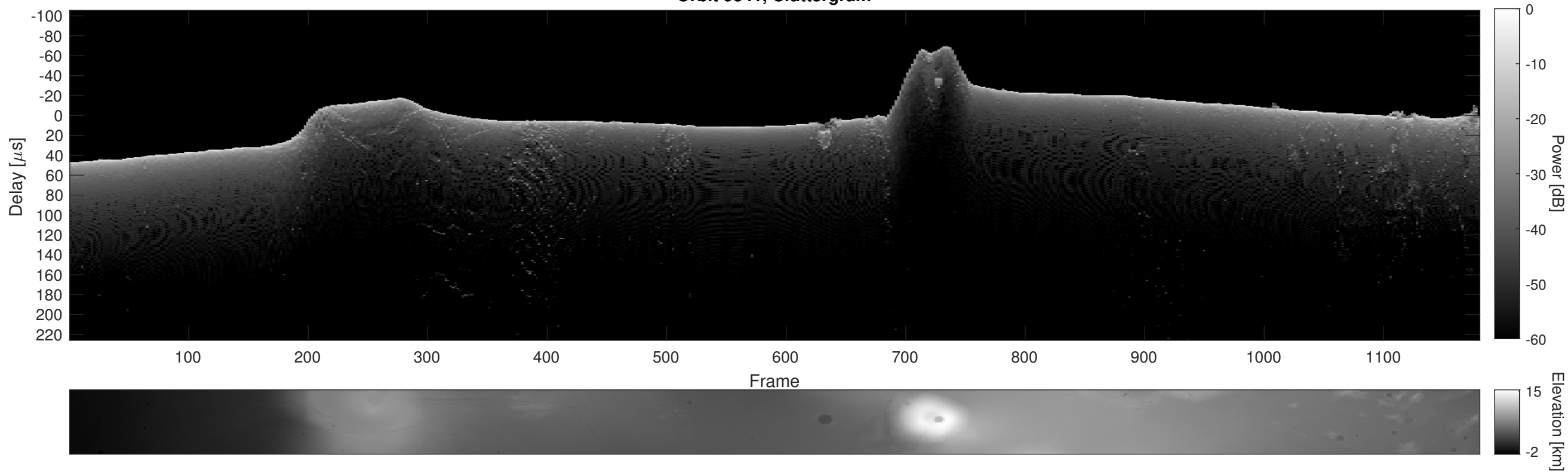
Orbit 9341, Cluttergram
