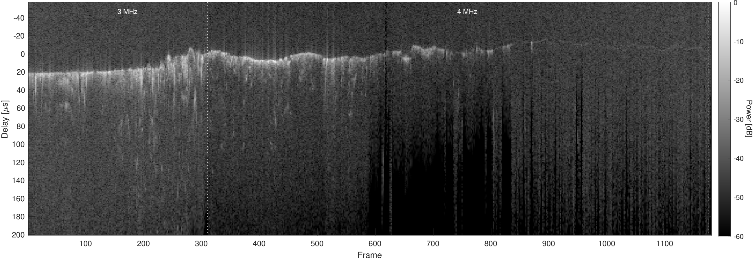
Orbit 9343, Optimized, No Window, Channel 2
